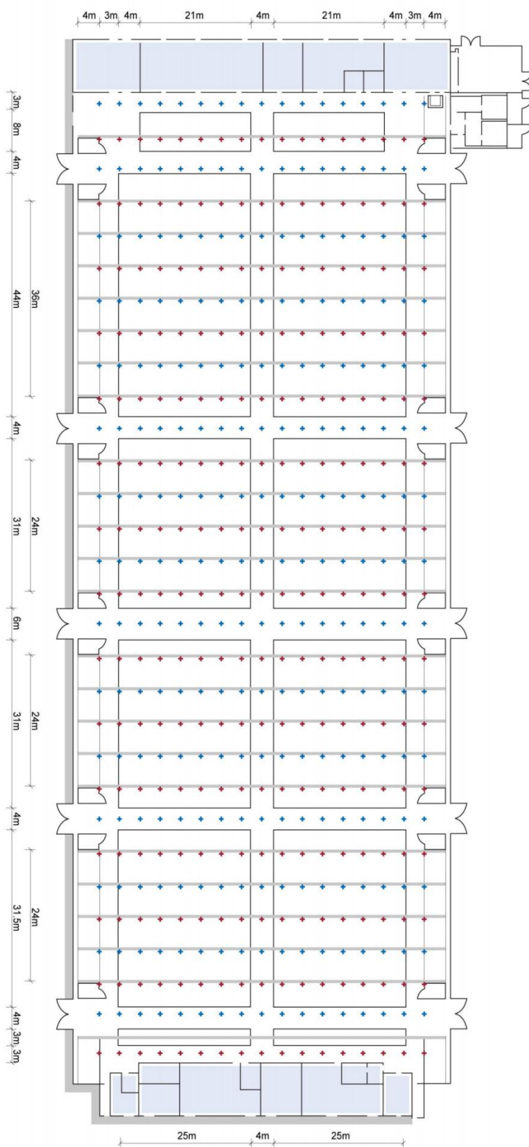
Standard Exhibition Layout in Halls N1 to N5 N1 至 N5 标准布展平面图
